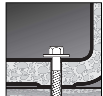
Bolt-down hardware
